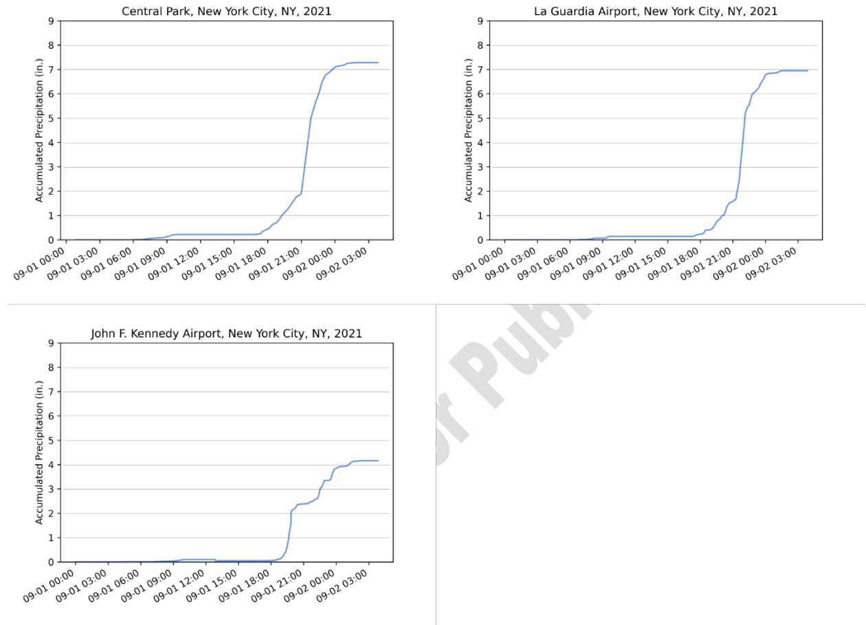
Figure 4. Observed accumulated precipitation at New York City Automated Surface Observing System (ASOS) weather stations during the Ida-remnants cloudburst (1-2 September 2021). Source: (ASOS data accessed through Iowa Environmental Mesonet, 2023a)
